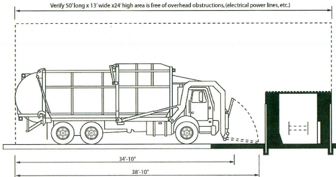
SIDE VIEW
